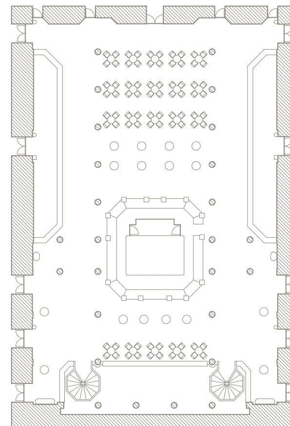
FOYER EBENE 2
